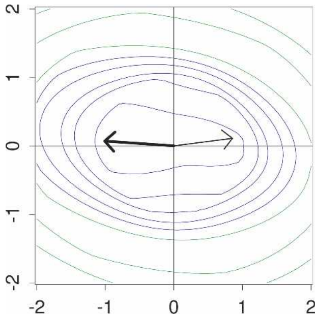
FIG. 11. The QuikSCAT objective function for a very low wind case. The example is cell 48 from the wind vector cell row presented in the previous figure (Fig. 10, top). The four observed \sigma^0 values multiplied by 10^6 and ordered as they were measured by QuikSCAT are outer fore, 56; inner fore, -40; inner aft, 42; and outer aft, -15.
