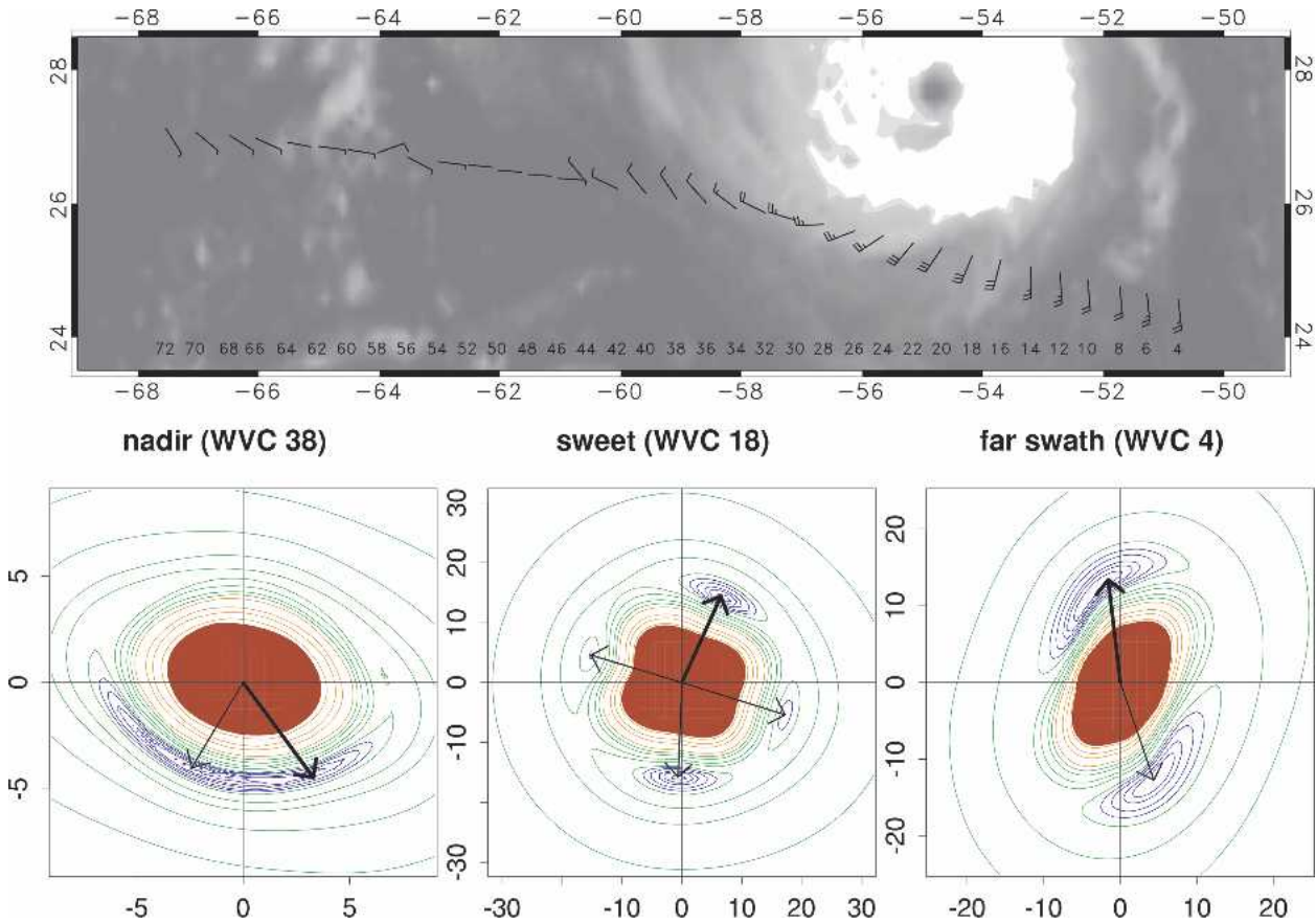
FIG. 10. The QuikSCAT objective function showing different ambiguity patterns. These data are for rev 6659, row 1100, and cells 38, 18, and 4. For reference the selected wind vectors for the even-numbered WVCs in row 1100 are plotted over the GOES imagery. Objective function plots as in Fig. 9a.
