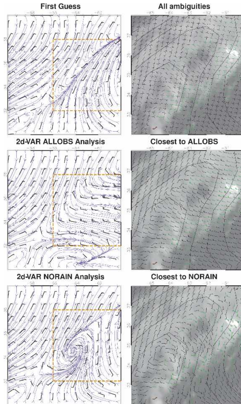
FIG. 8. An example of the impact of QuikSCAT data on a variational analysis. (upper left) A portion of the background wind field used in 2DVAR in the vicinity of a synoptic front. The background field is a 3-h NCEP GFS forecast, valid at 2100 UTC 28 Sep 2000. Streamlines are plotted to highlight instantaneous features in the flow; the 2DVAR (middle) ALLOBS and (lower left) NORAIN analyses, respectively. (right) The area of the orange-dashed boxes drawn in the left panels and the QuikSCAT ambiguities over the GOES image and the sea level pressure analysis of Fig. 4 except that the contour interval is 0.5 hPa. (top left) The directions, but not speeds, for all ambiguities; the ambiguities closest to the (middle) ALLOBS and (lower left) NORAIN analyses, respectively. Rain-flagged winds are green.
