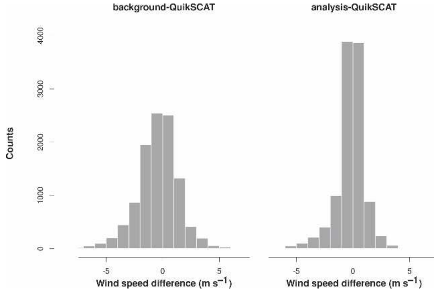
FIG. 7. Histograms of differences of QuikSCAT-selected winds from (left) the background and (right) the NORAIN 2DVAR analysis.
