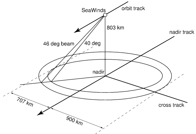
FIG. 3. A schematic of the measurement geometry of the SeaWinds instrument on board QuikSCAT (from Freilich 2000). As indicated in the figure the far swath extends from 700 to 900 km on either side. The nadir swath is 400 km wide, centered on nadir.
