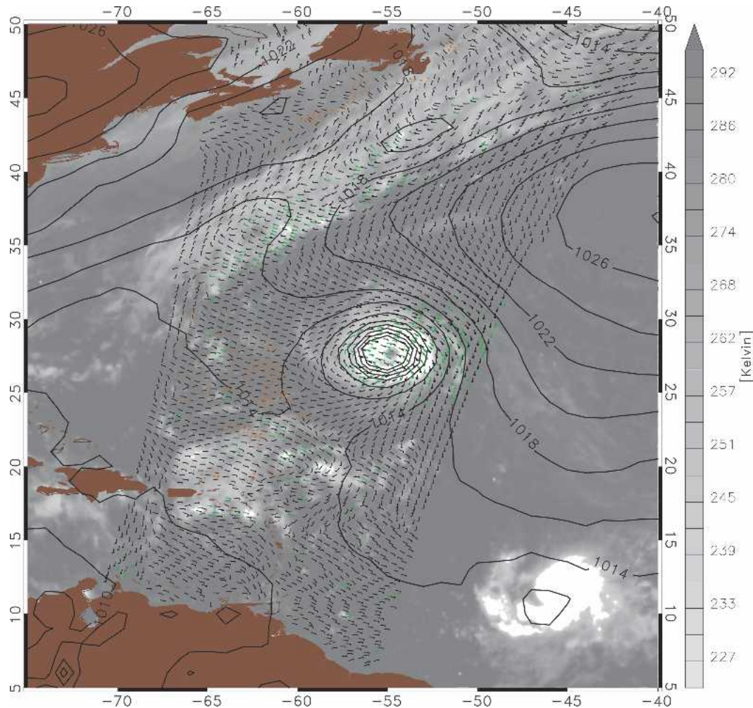
FIG. 4. QuikSCAT winds, NCEP GFS sea level pressure analysis, and GOES infrared imagery over the western North Atlantic close to 2200 UTC 28 Sep 2000. The QuikSCAT data swath represents about 12 min of data collected during rev 6659 centered at 2207 UTC. Winds are plotted using standard wind barb notation with short, long, and filled triangle flags indicating 5, 10, and 50 kt ( 2.57 , 5.14 , and 25.72 \text{m s}^{-1} ). Rain-flagged winds are green. Red dots indicate the locations of negative \sigma^p observations. For clarity the QuikSCAT winds have been thinned to every fourth WVC along and across track. The NCEP GFS MSLP analysis valid at 0000 UTC 29 Sep is contoured every 2 hPa. The GOES image valid at 2215 UTC is shaded according to the grayscale on the right.
