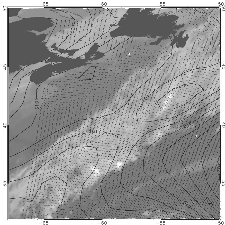
FIG. 6. Same as in Fig. 4 but for winds around a front in the northwestern North Atlantic at full resolution.
