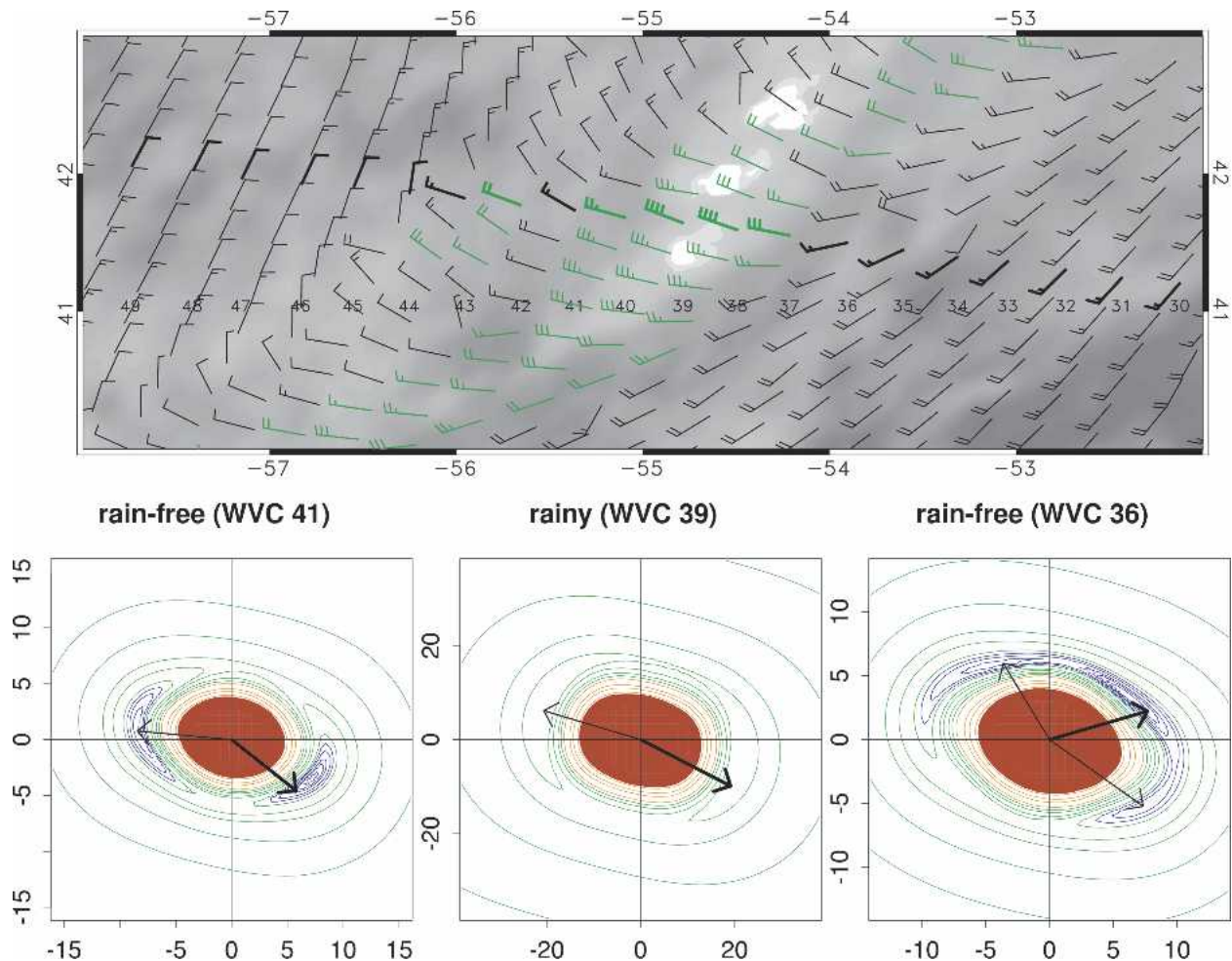
FIG. 12. An example of rain-contaminated winds from QuikSCAT. (top) The vector cell row of interest is shown in bold wind barbs. Rain-flagged winds are green. (bottom) The QuikSCAT objective function for cells 41, 39, and 36.
